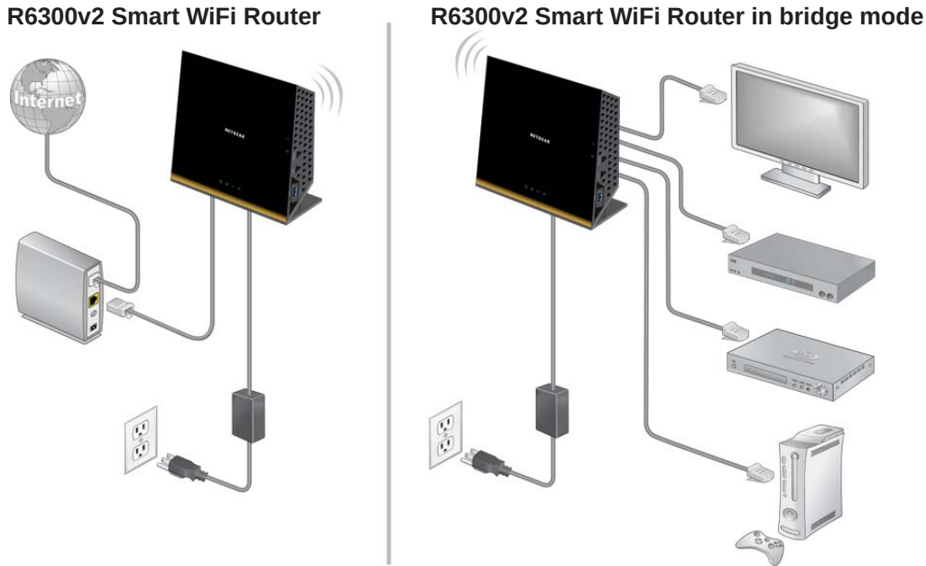
Figure 8. Router in bridge mode with an 802.11ac WiFi connection
